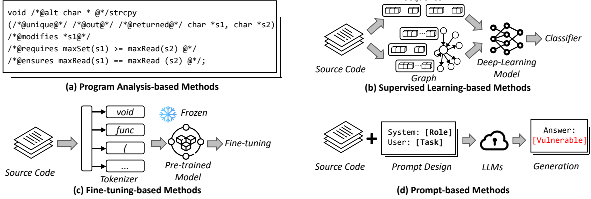
Figure 2: The four types of vulnerability detection methods.
