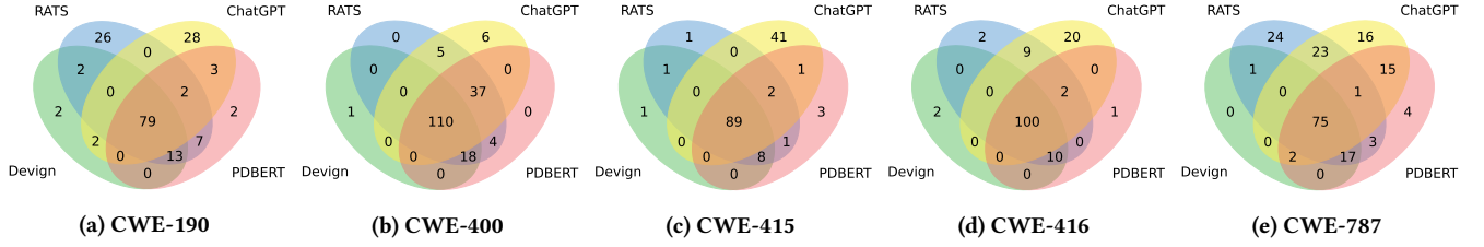
Figure 4: The experimental results of several vulnerability types, including CWE-190, CWE-400, CWE-415, CWE-416, and CWE-787. The green, blue, red, and yellow circles denote the results of Devign, RATS, PDBERT, and ChatGPT, respectively.
