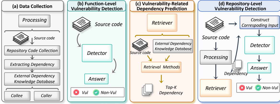
Figure 3: The overview of VulEval. Figure (a), (b), (c), and (d) denote the process of data collection, function-level vulnerability detection, vulnerability-related dependency prediction, and repository-level vulnerability detection, respectively.
